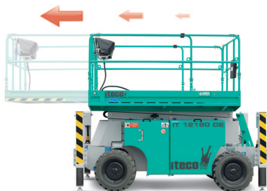
Manual deck extension 1.4 m
